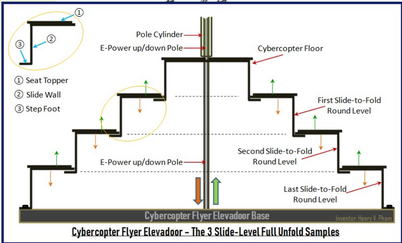
Figure-012: Cybercopter Flyer – 3-Level Foldable Round Seats Elevador Full-unfold Sample
