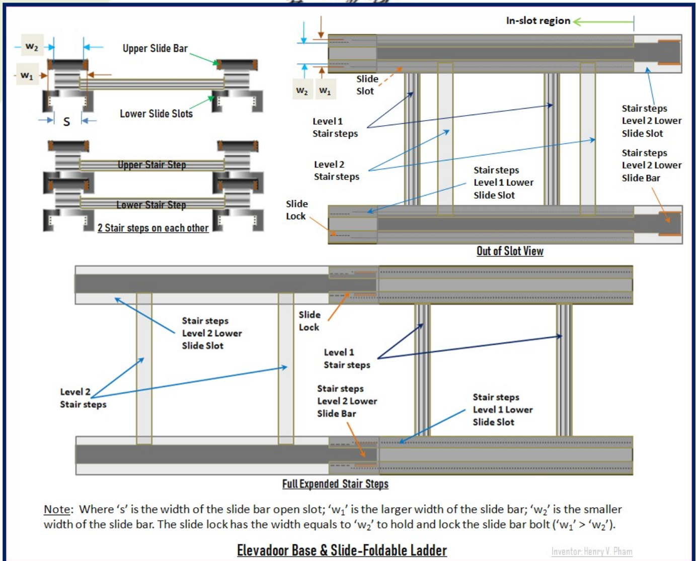
Figure-05: Cybercopter Flyer – Elevador Base & Slide-Foldable Ladder Details
