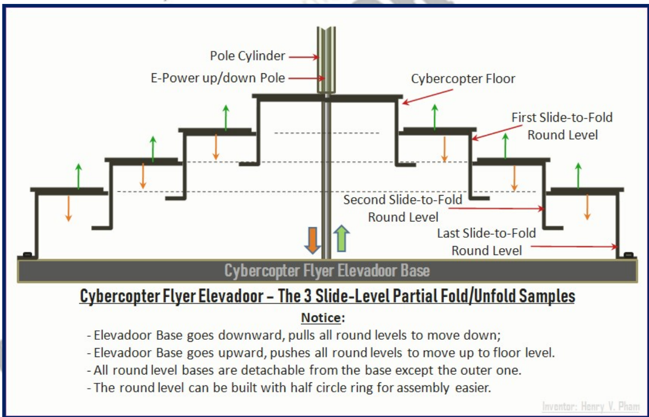
Figure-013: Cybercopter Flyer – 3-Level Foldable Round Seats Elevador Partial Fold/Unfold Sample
