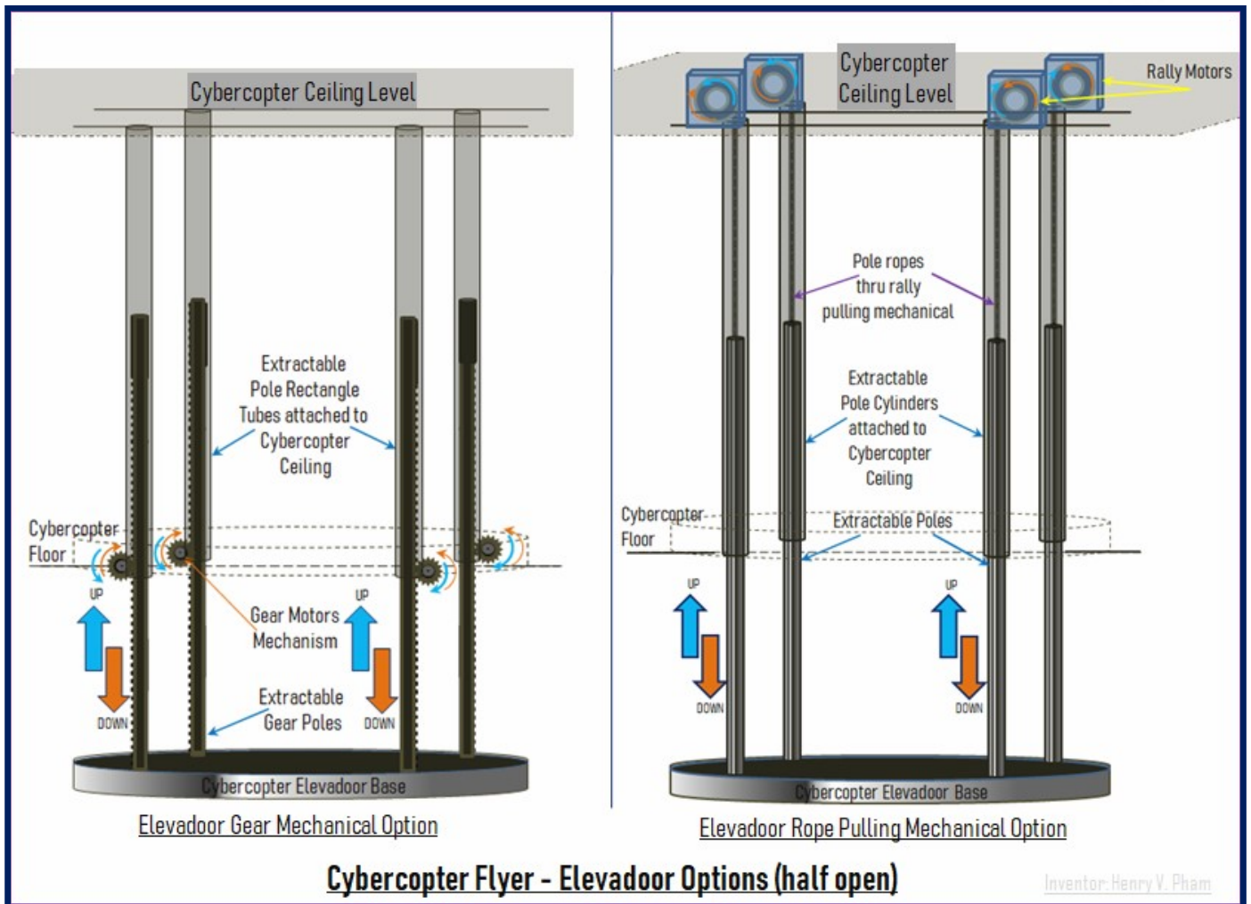
Figure-01: Cybercopter Flyer -Elevadoor Options (half open view)
