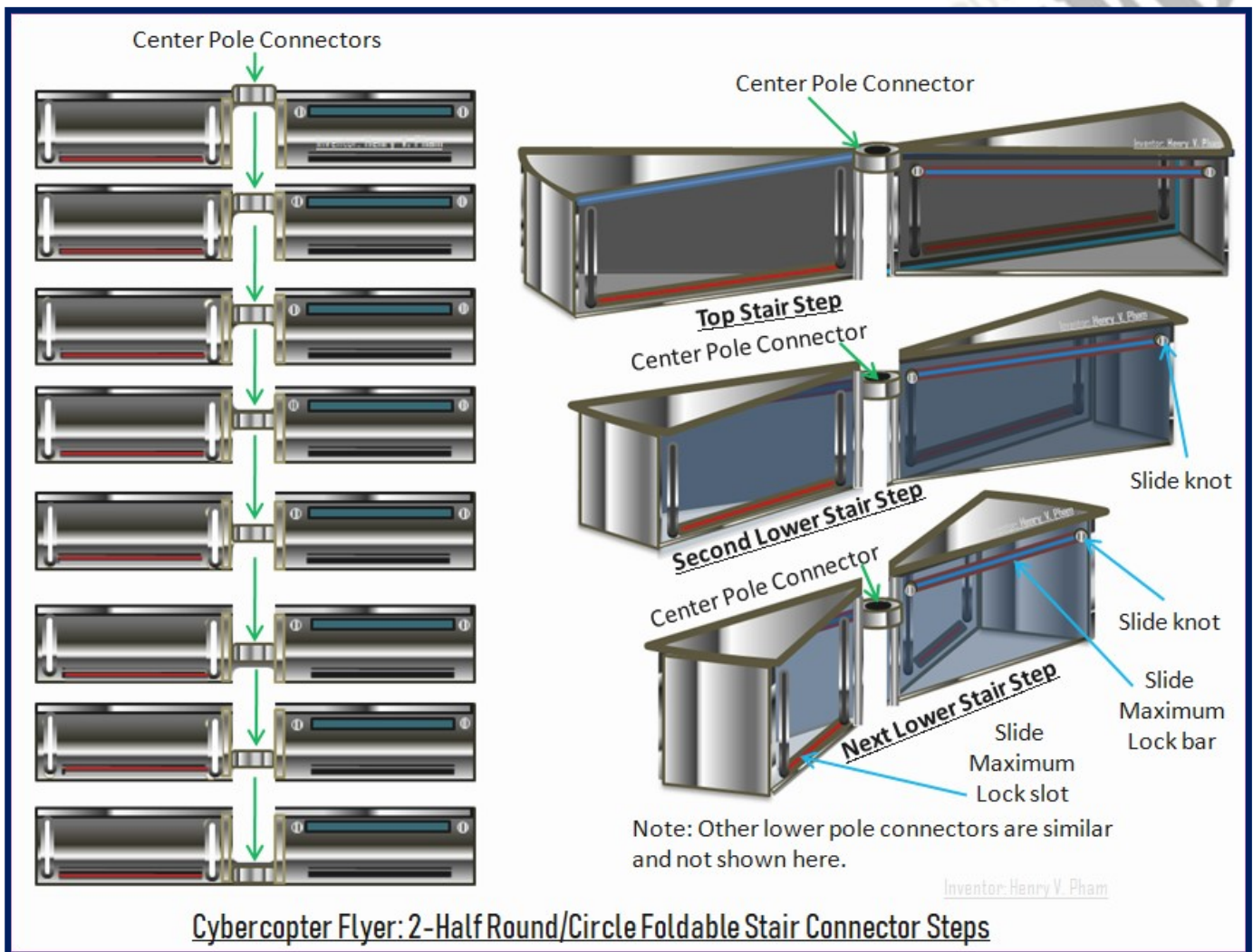
Figure-010: Cybercopter Flyer – 2-Half Circle Foldable Stair Connector Steps
